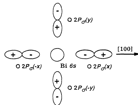
FIG. 3. Illustration of the nonbonding wave function \phi_1 , which has d(x^2-y^2) symmetry. The amplitude of this wave function is zero along the [110] direction, which results in the weaker forbidden transition [110].
