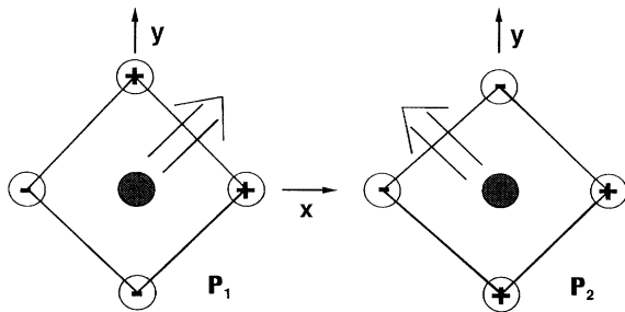
FIG. 4. Two small excitons in the x - y plane with a p symmetry. The exciton consists of a quasiparticle (solid circle) at sublattice A and a linear combination of four nearest neighbor quasiholes (hollow circle) state at sublattice B . The signs indicate the relative phases of quasiholes. The arrows indicate the directions of the exciton motion with the strongest oscillator strength.
