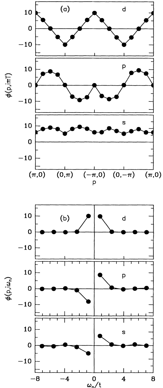
FIG. 4. Monte Carlo results for the leading eigenfunctions in the pairing channel, \phi_d(\mathbf{p}, i\omega_n) , \phi_p(\mathbf{p}, i\omega_n) , and \phi_s(\mathbf{p}, i\omega_n) , on an 8\times 8 lattice with U=8t and T=0.25t . (a) Momentum structure of the leading eigenfunction for \omega_n=\pi T . Here \mathbf{p} is taken along the path shown in the inset of Fig. 3(a). (b) Frequency structure of the leading eigenfunctions. Here \phi_d(\mathbf{p}, i\omega_n) and \phi_s(\mathbf{p}, i\omega_n) are shown for \mathbf{p}=(\pi, 0) , and \phi_p(\mathbf{p}, i\omega_n) is shown for \mathbf{p}=(\pi/2, \pi/2) .
