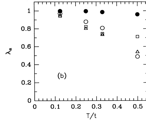
FIG. 2. Eigenvalues of the Bethe-Salpeter equations vs T for (a) U=4t and (b) U=8t for an 8 \times 8 half-filled lattice. The solid points are for the \mathbf{Q}=(\pi,\pi) antiferromagnetic particle-hole eigenvalue of Eq. (3). The open symbols denote the eigenvalues of the \mathbf{q}=(0,0) particle-particle Bethe-Salpeter Eq. (4) with ( \circ ) corresponding to the singlet d_{x^2-y^2} even-frequency amplitude, ( \triangle ) to a singlet, odd-frequency p -wave amplitude, and ( \square ) to a triplet, s -wave odd-frequency amplitude.
