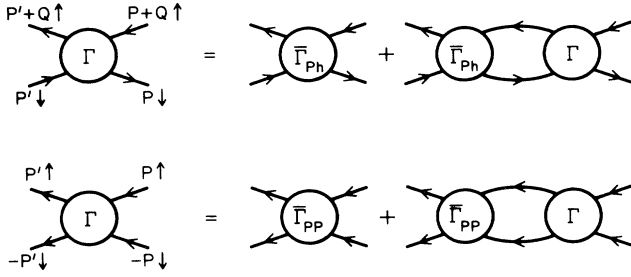
FIG. 1. The particle-hole and particle-particle t -matrix equations. Here the lines represent dressed single-particle propagators and \mathbf{Q}=(\pi,\pi) . \Gamma is the two-fermion scattering vertex, and \bar{\Gamma}_{ph} and \bar{\Gamma}_{pp} are the irreducible particle-hole and particle-particle vertices, respectively.
